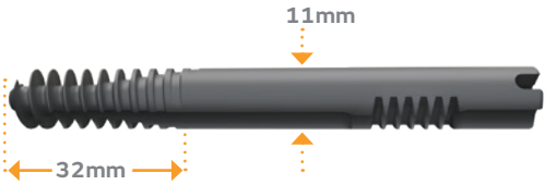
Minor diameter tapers from 11-5.6mm
