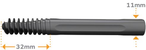
Minor diameter tapers from 11 to 5.6mm Subtrochanteric Lag Screw 70-125mm length
